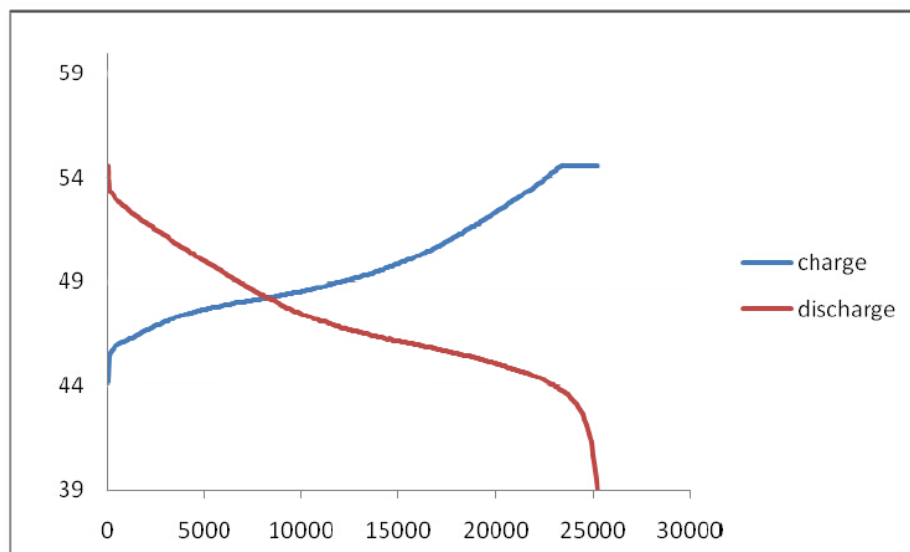
48V24Ah Charge-Discharge Curve ( 0.2C, 25°C )
